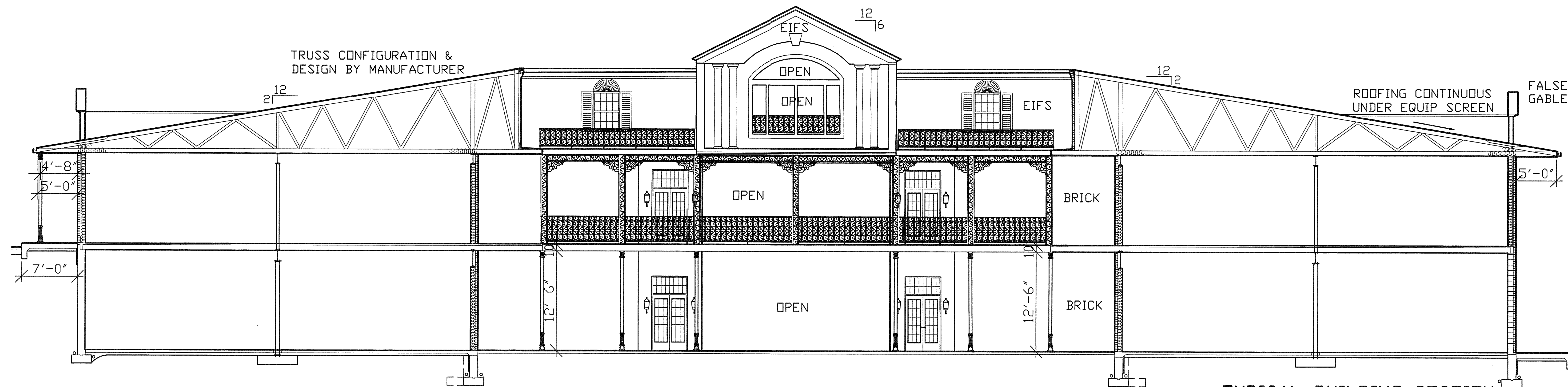
TYPICAL BUILDING SECTION SCALE: 1/4" = 1'-0"
