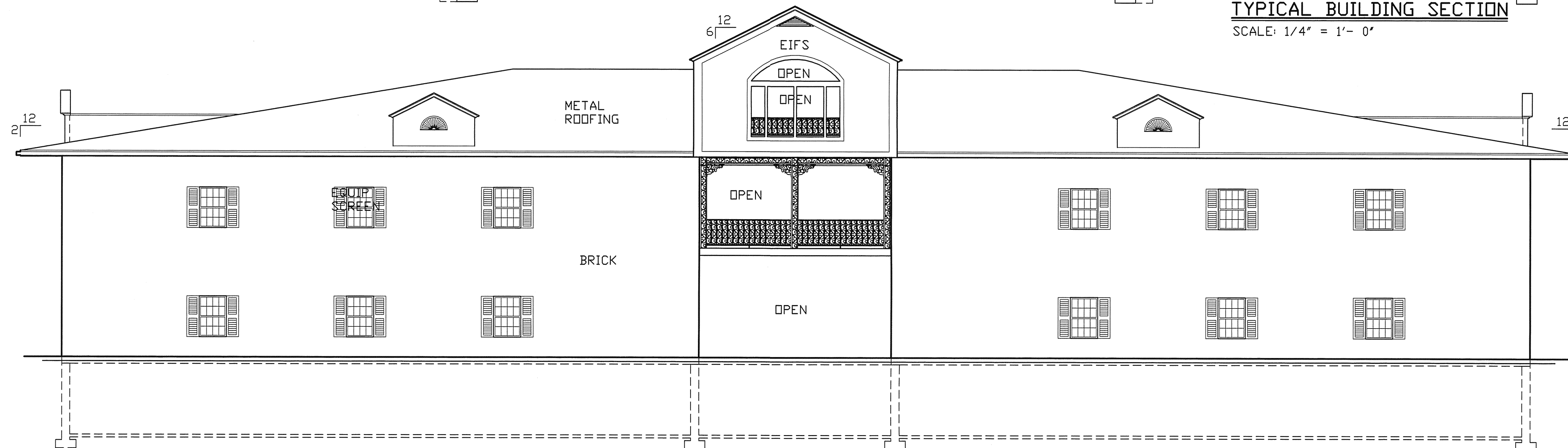
PARKING LOT - LOOKING WEST SCALE: 1/8" = 1'-0"
