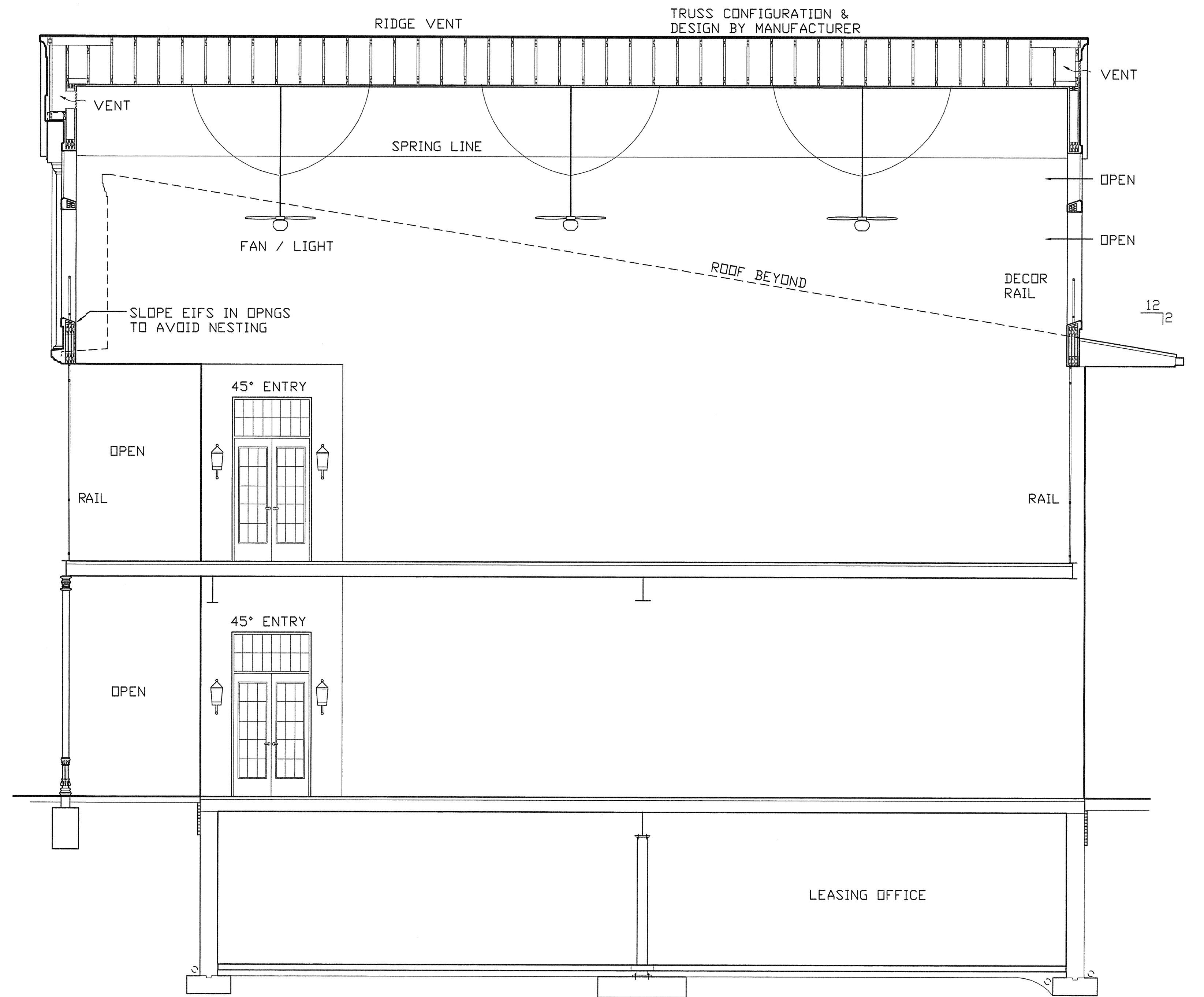
CENTER WALK-THRU SCALE: 1/4" = 1'-0"
