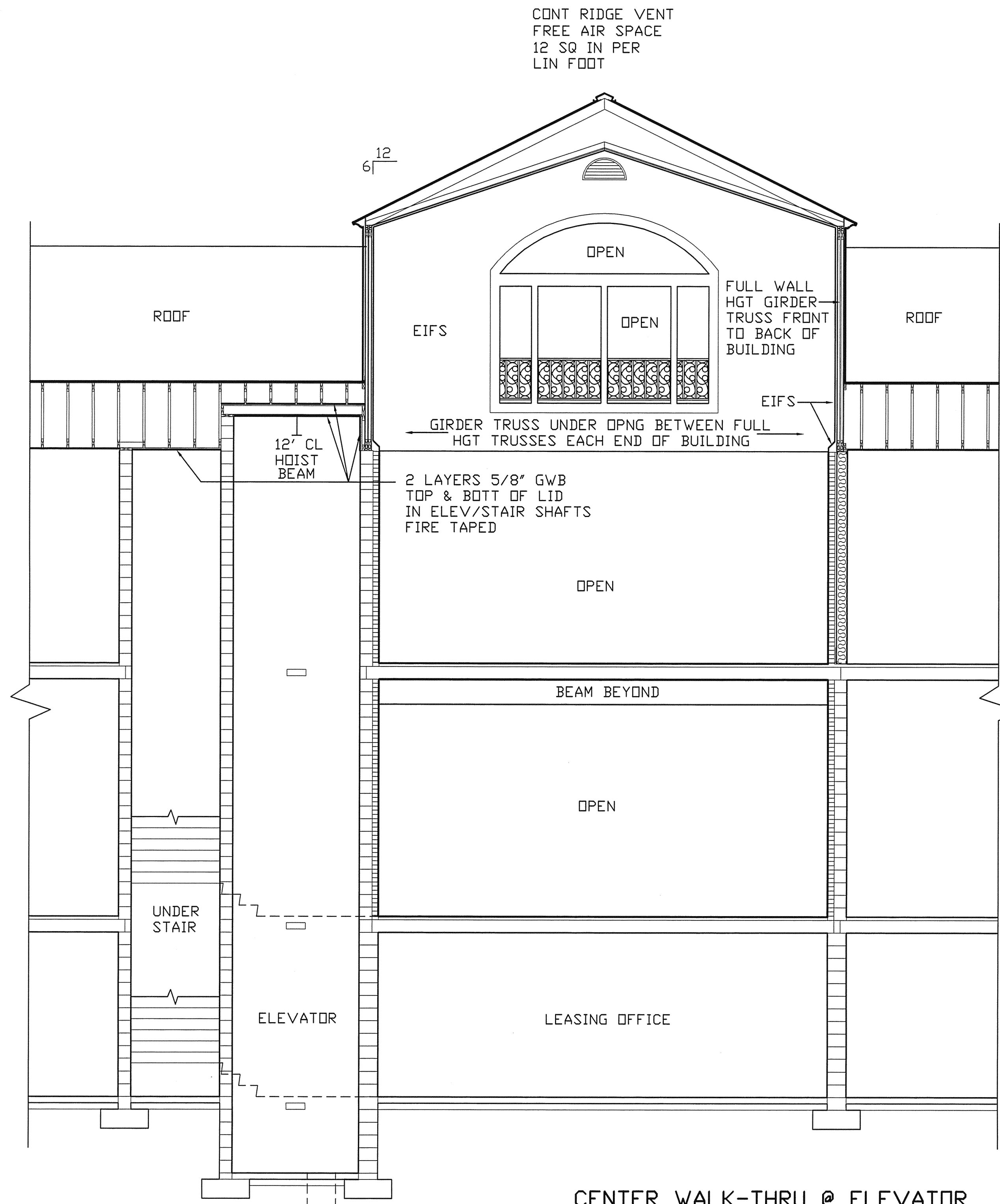
CENTER WALK-THRU @ ELEVATOR SCALE: 1/4" = 1'-0"
